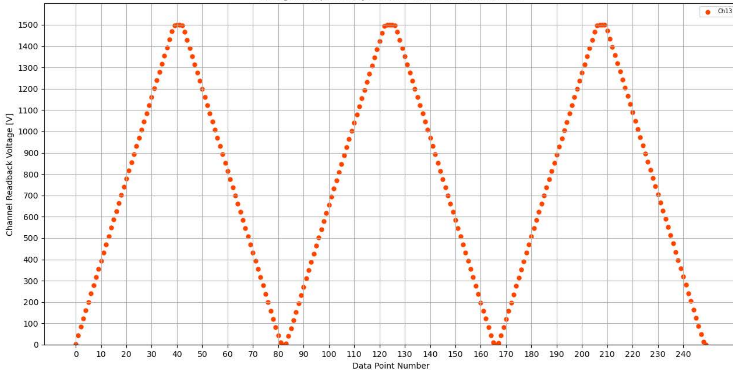
Voltage Ramp Test (Python) Bd #358, Slot #6, Ch #13
