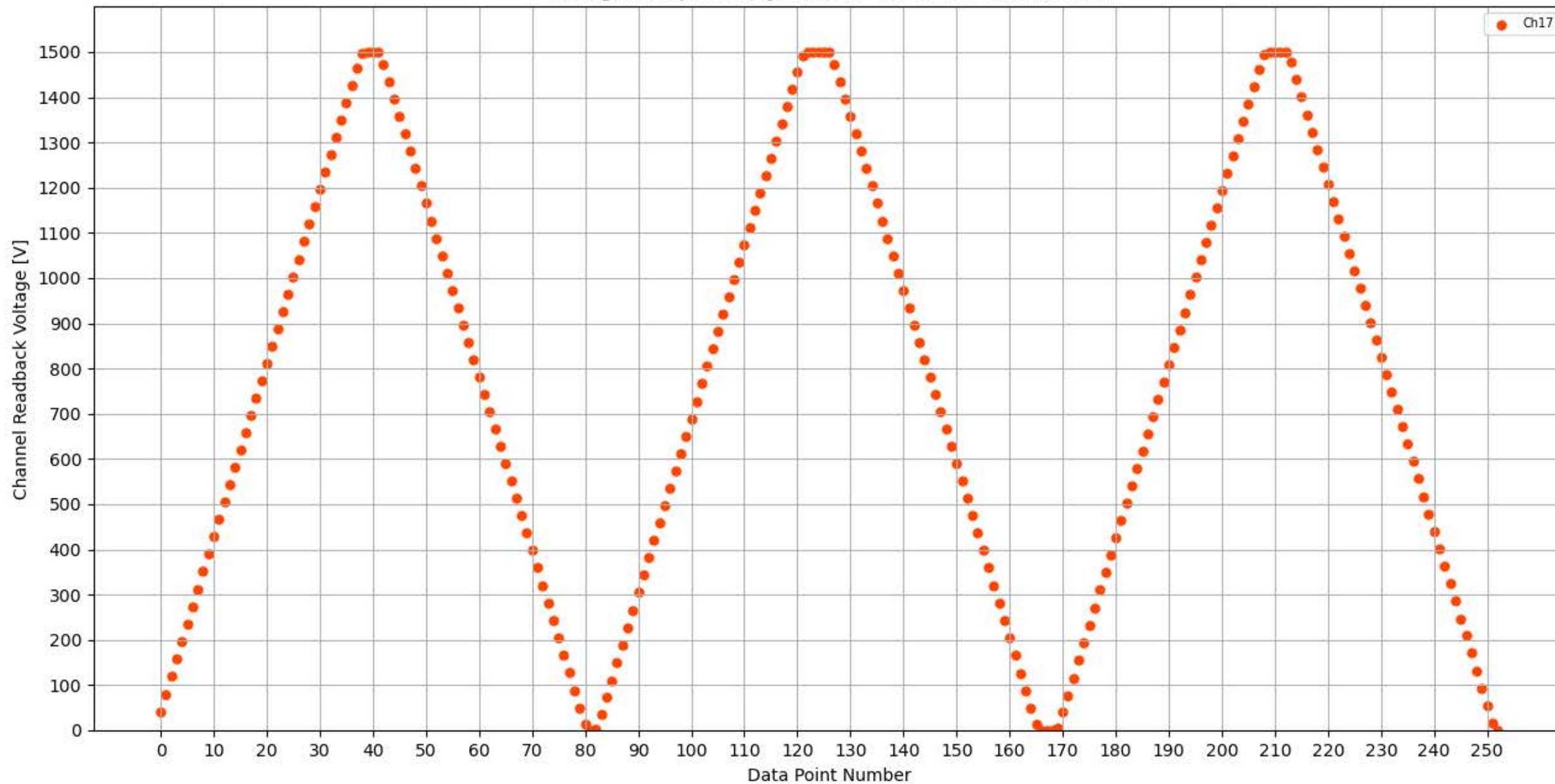
Voltage Ramp Test (Python) Bd #358, Slot #6, Ch #17
